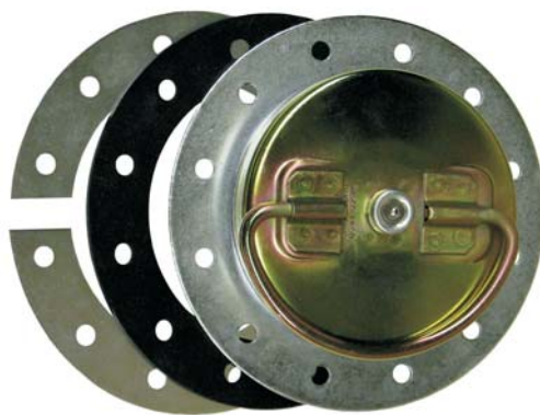
600 Series Cap with Flanged Neck, Gasket and split Mounting Ring
